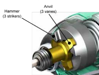
Mechanism of the Triple Hammer
