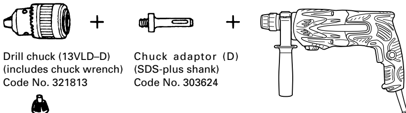
Chuck wrench
