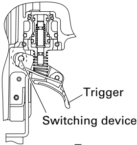
Enlarged view of the valve part
