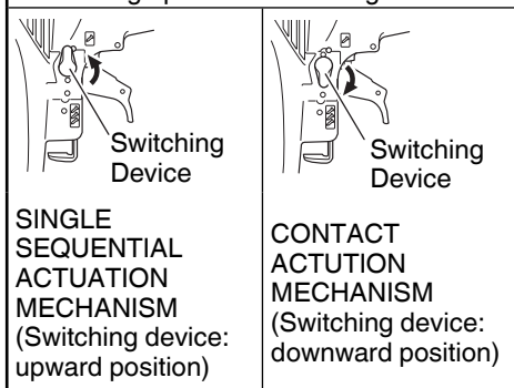
Nailing operation Switching device
