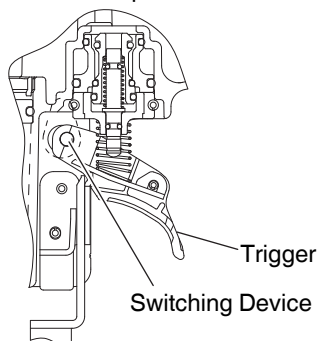
Enlarged view of the valve part
